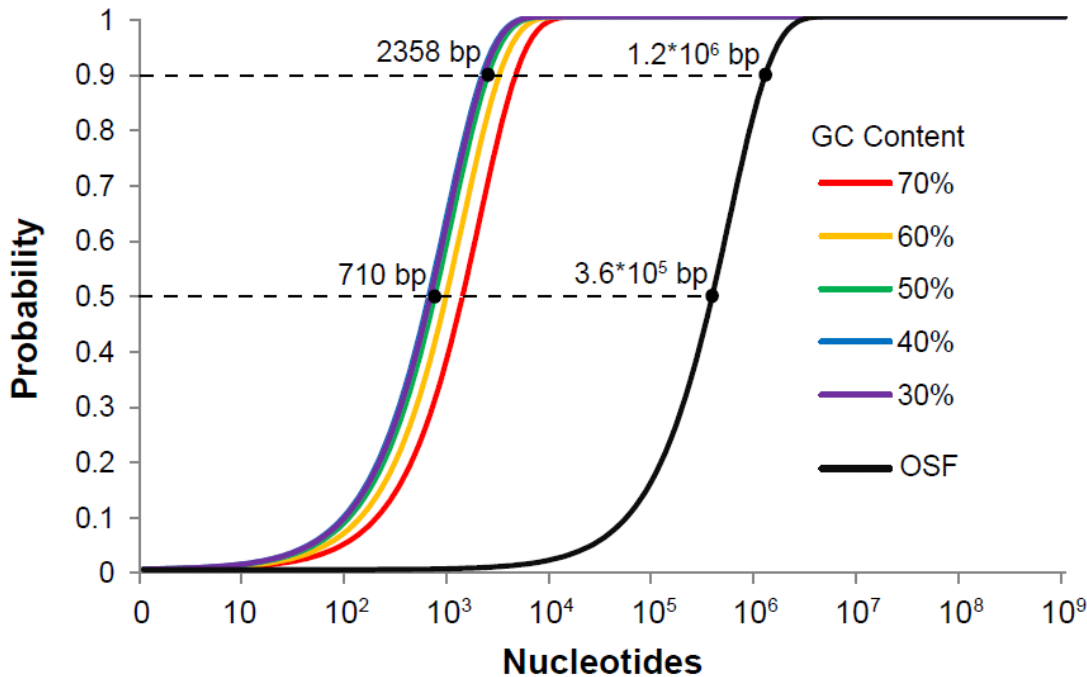
Fig. 3: Comparison between the probability of the occurrence of homing endonuclease sites RFC[95] and the current BioBrick RFC[10] restriction sites in a sequence of a given length.
