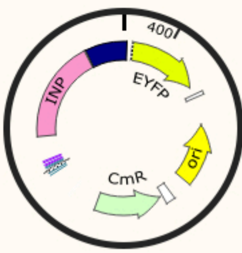
INP-Streptavidin-YFP_2 4918 bp
