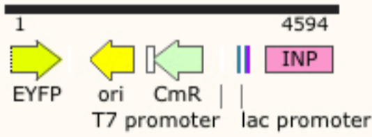
INP-strepta-YFP-after-PCR-with-gibson-primers 4594 bp
