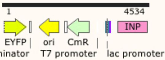
INP-Strepta-YFP-after-adding-linker 4534 bp
