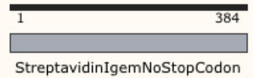
Strepta-igem-whithout-stop-codon 384 bp
