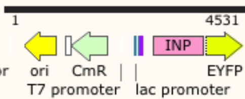
INP-YFP-Strepta-PCR-linker 4531 bp
