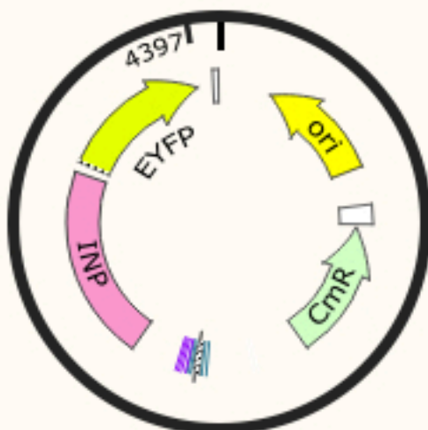
pBS1C3YFP 4516 bp
