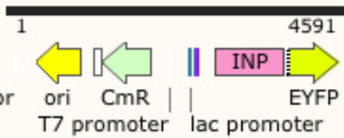
INP-YFP_Strepta-linker-a...PCR-with-Gibson-primers 4591 bp
